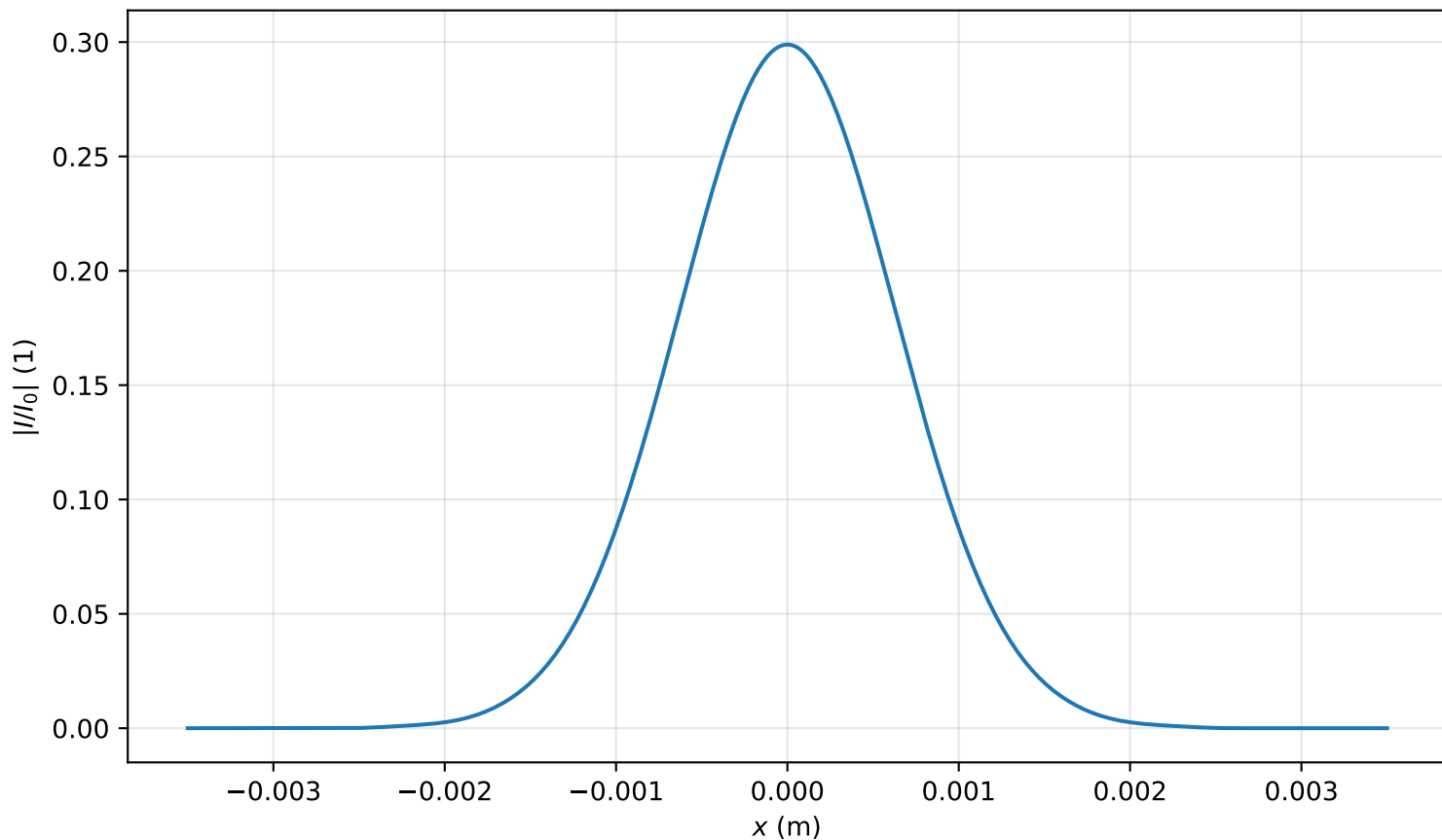
Intensity profile I(x, y = 0, z = 3.264m)/I_0 , P_{in}=0.1P_{cr} , artificial time
